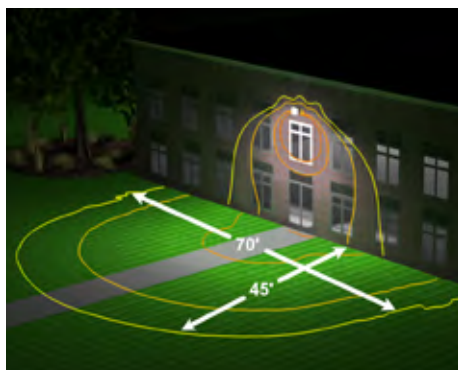
80W fixture mounted at 20' with narrow distribution
