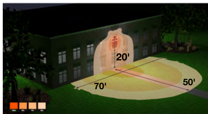
80W fixture mounted at 20' with Type IV distribution
