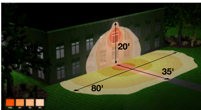
80W fixture mounted at 20' with a Type II distribution
