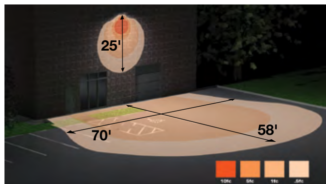
60W fixture mounted at 25' with a 30° tilt
