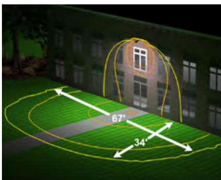
60W fixture mounted at 20' with Type II distribution
