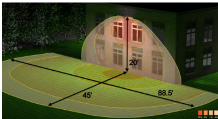
100W fixture mounted at 20'
