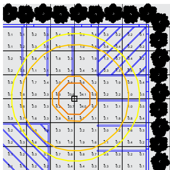
50W fixture mounted at 10'
