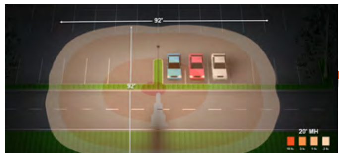
80W fixture mounted at 20' with Type V distribution
