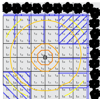
50W fixture mounted at 14'
