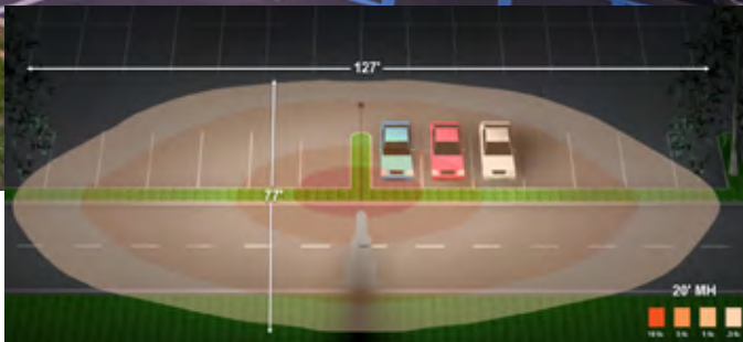
80W fixture mounted at 20' with Type II distribution
