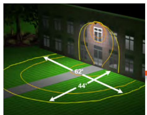
60W fixture mounted at 20' with Type IV distribution
