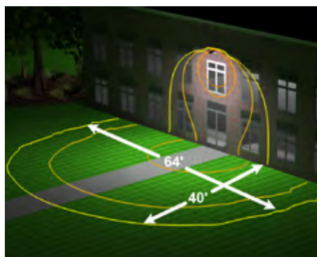
60W fixture mounted at 20' with Type III distribution
