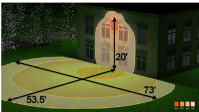
80W fixture mounted at 20'
