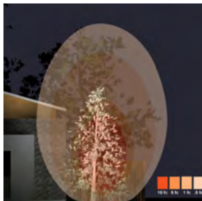
30W, 6' setback, 60° tilt, 25° beam spread
