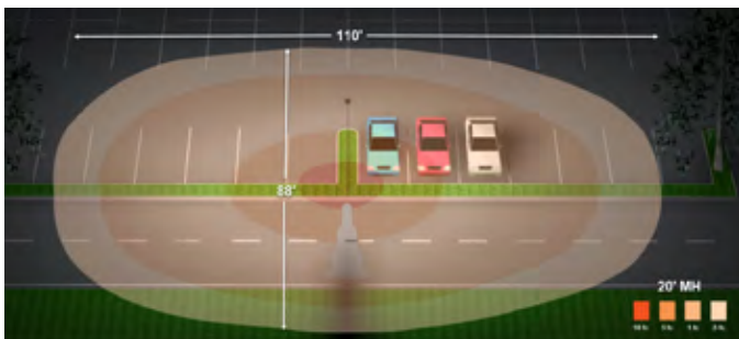
80W fixture mounted at 20' with Type IV distribution
