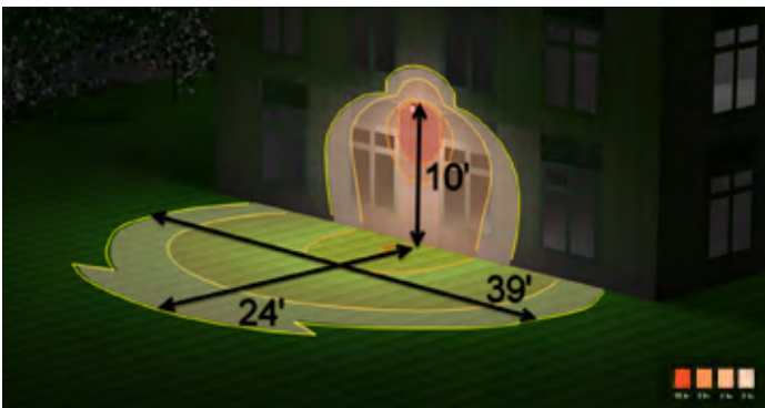
30W fixture mounted at 10'
