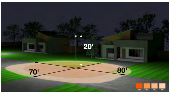
90W fixture mounted at 20' with Type IV Distribution
