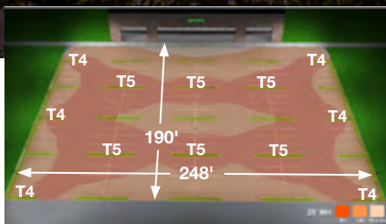
190W fixture mounted at 25' with Type IV and V Distribution
