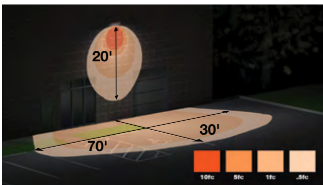
60W fixture mounted at 20'
