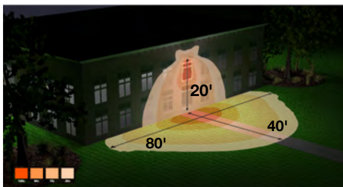
80W fixture mounted at 20' with Type II distribution
