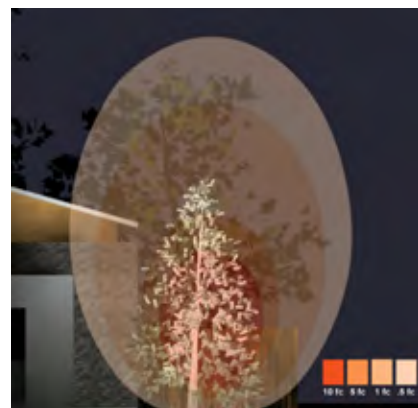
30W, 6' setback, 60° tilt, 40° beam spread
