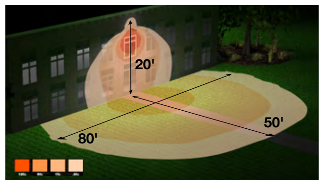
80W fixture mounted at 20' with a Type IV distribution
