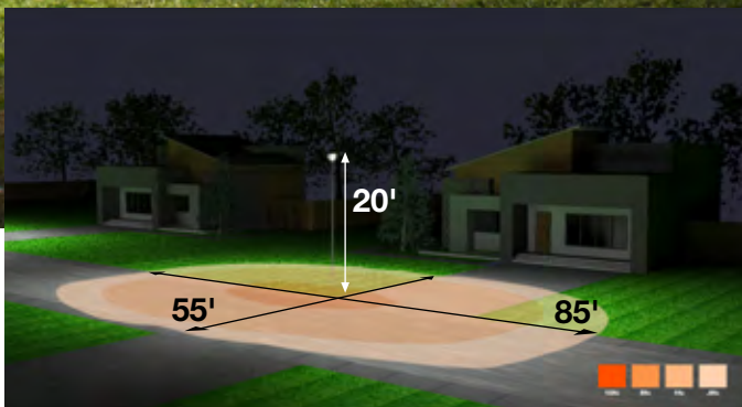
90W fixture mounted at 20' with Type II Distribution
