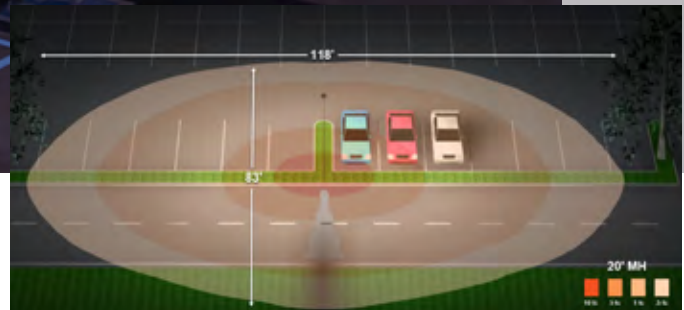
80W fixture mounted at 20' with Type III distribution
