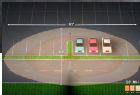
80W fixture mounted at 20' with Type IV distribution
