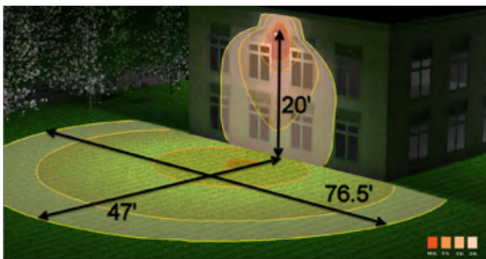
80W fixture mounted at 20'
