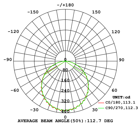
65793, 12W
