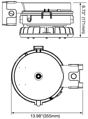
HIGH BAY 80W, WALL MOUNT
