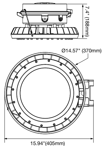
HIGH BAY 150W & 200W, WALL MOUNT
