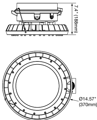
HIGH BAY 150W & 200W, 25° STANCHION MOUNT
