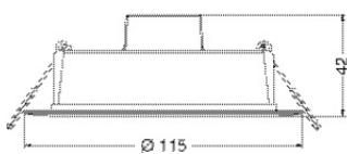
DL IP44 DN 115 8W
