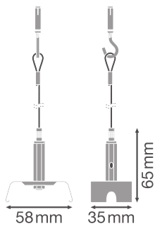
TRUSYS FLEX SUSPENSION KIT
