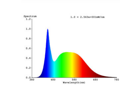
RGBW Remote Lamp 6500K
