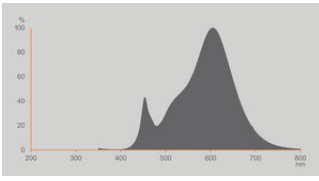
Spectral graph classic A 2700K MS/DS
