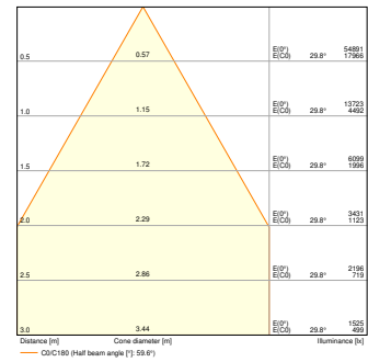
HB P 75W 840 70DEG IP66 PS - REFLECTOR
