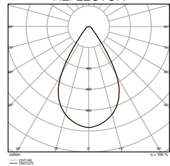
HB P 75W 840 70DEG IP66 PS set to 53W
