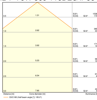
HB P 75W 865 110DEG IP66 PS set to 53W
