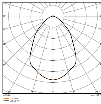
HB P 75W 865 110DEG IP66 PS - REFRACTOR
