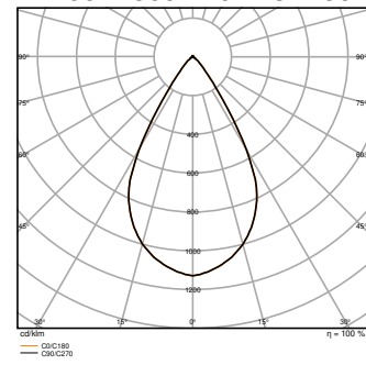
HB P 75W 865 110DEG IP66 PS - REFLECTOR
