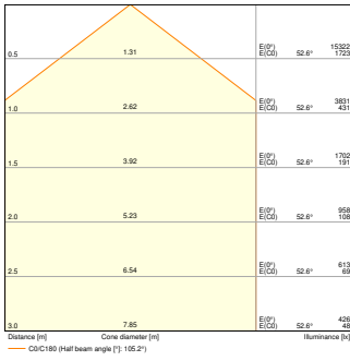
HB P 53W 865 110DEG IP66 PS
