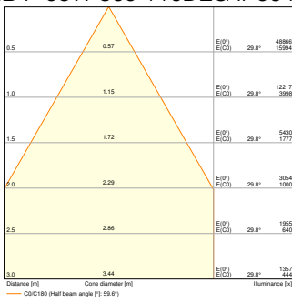
HB P 75W 865 110DEG IP66 PS - REFLECTOR
