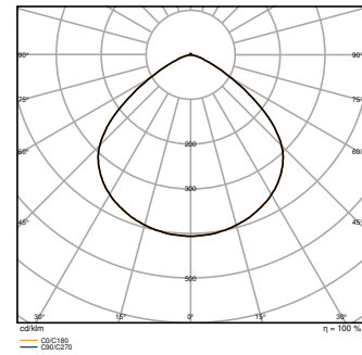
HB P 53W 865 110DEG IP66 PS
