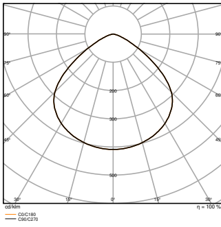
HB P 75W 865 110DEG IP66 PS
