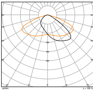
FL FLEX P 80W ML 840 A45X140 WAL LEDV
