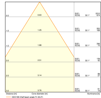
SP CBO FPFIX V 6W MS840 DIM IP65 WT
