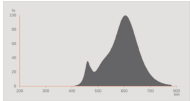
LISO spectral power distribution 2700K CRI80 v1
