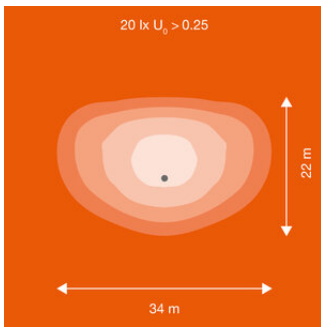
Floodlight Performance 150W ASYM 45x140 simplified isolux diagram
