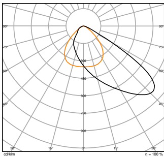
FL AREA 105W 840 ASYM 48X92 BK
