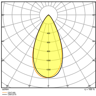
LEDV DL PFM SURFACE 20W 840 50
