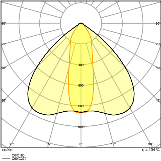
LEDV LOWBAY 100W 850 HRO 30X90
