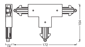
TRACKLIGHT T CONNECTOR
