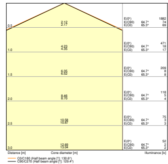
SF SQUARE 330 V 24W 3CCT 4000K IP44
