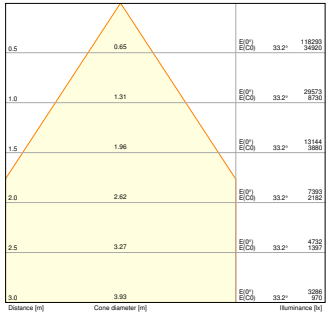
HB P 200W 865 70DEG IP66 PS - REFLECTOR
