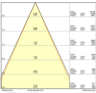
TR SP ZOOM DIM P 30W 940 WT 50D
