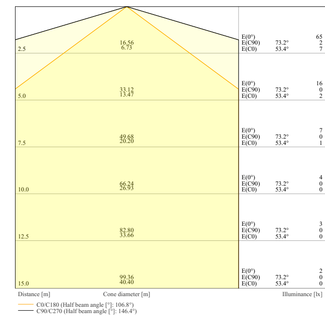
LISOEV 1465X31 25 17W 940 S130 LEDV 350mA
