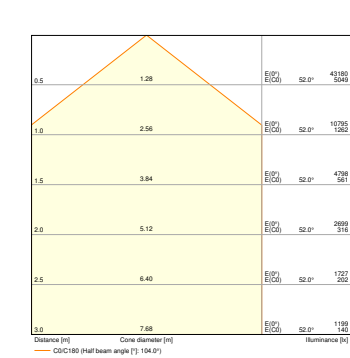
HB P 150W 865 110DEG IP66 PS
