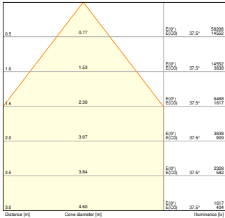
HB P 150W 865 110 DEG IP66 PS - REFRACTOR
