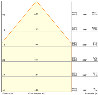
HB P 150W 865 110 DEG IP66 PS - REFLECTOR
