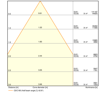
HB DA P 200W 840 70DEG IP66 WITH REFLECTOR
