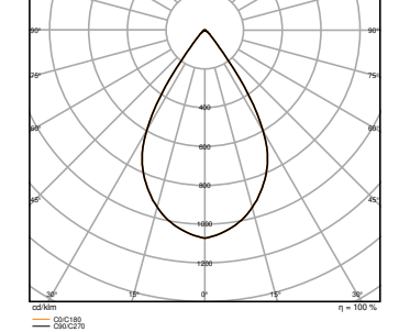
HB DA P 200W 840 70DEG IP66 WITH REFLECTOR
