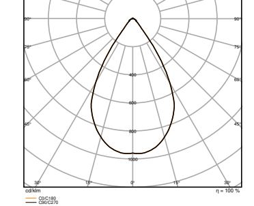
HB DA P 200W 840 70DEG IP66 WITH REFRACTOR
