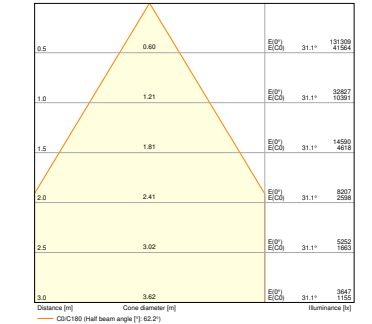
HB DA P 200W 840 70DEG IP66 WITH REFRACTOR
