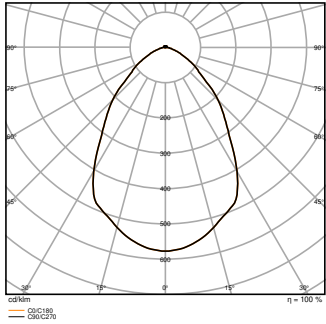
HB DA P 150W 865 110DEG IP66 WITH REFRACOR
