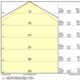
LB FLEX 1500 P 73W 840 VW WITH BP COVER
