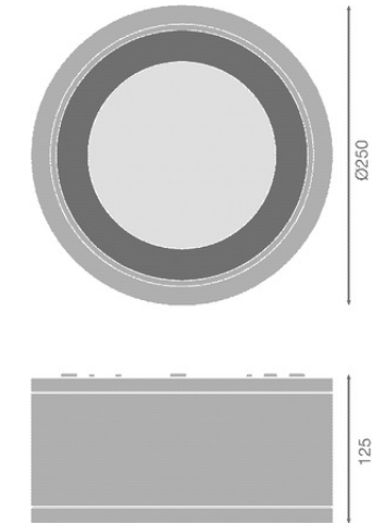
DL SURFACE DN250P 45W IP65 WT
