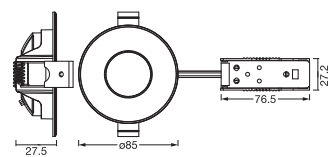
SPOT SET 4.9W 827 120DEG
